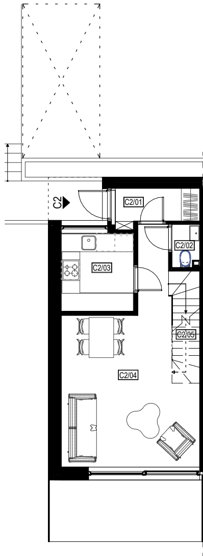
PARTER
